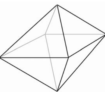
octahedron
