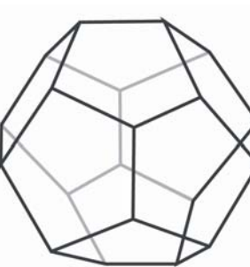
dodecahedron
