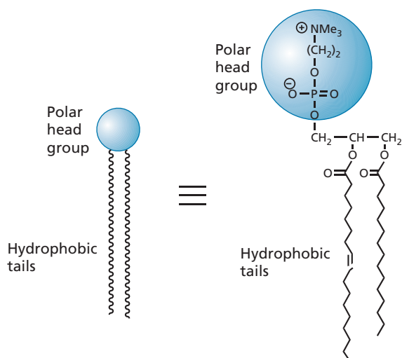
FIGURE 1.2 Phosphoglyceride structure.
