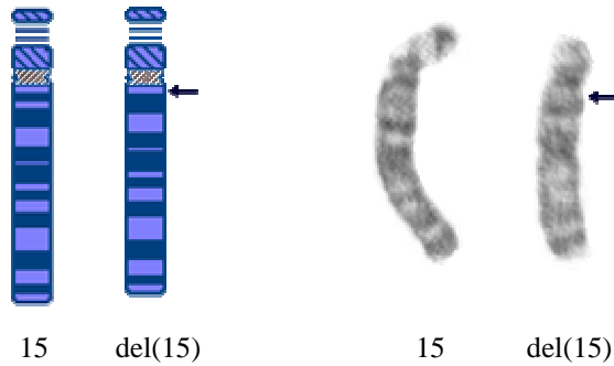
G-banding
